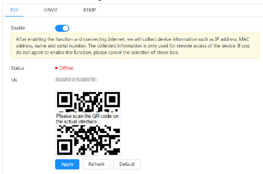
Figure 4-45 P2P
