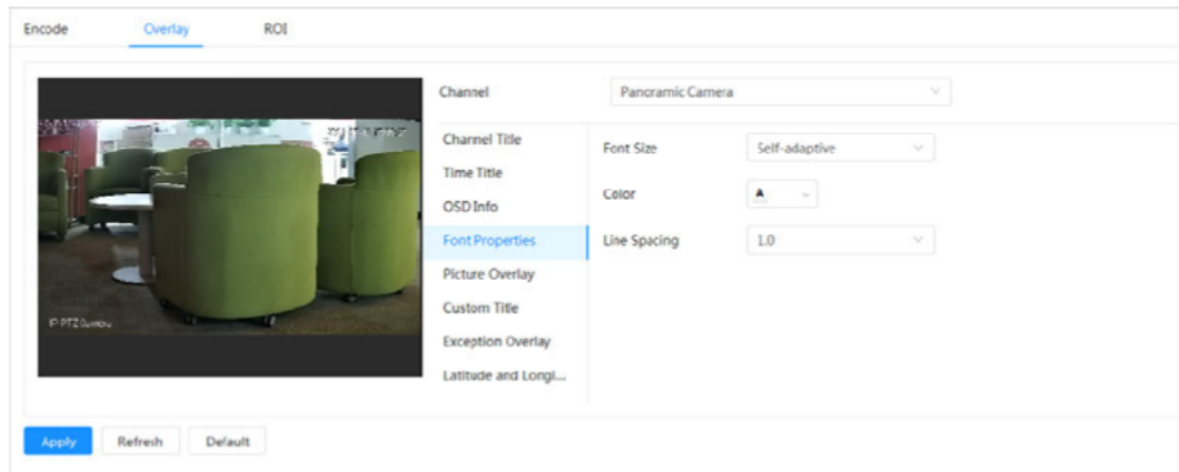
Figure 4-21 Font properties
