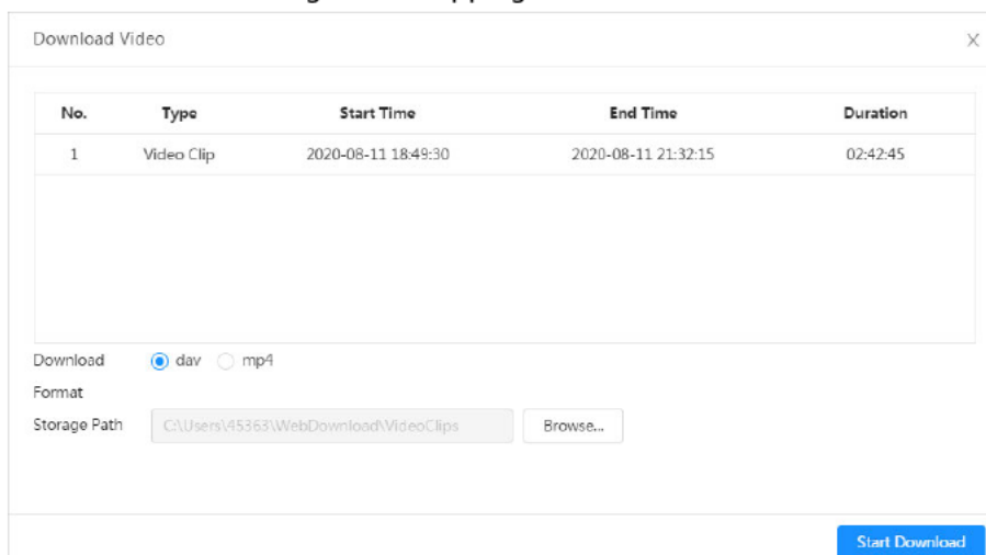
Figure 6-4 Clipping video
