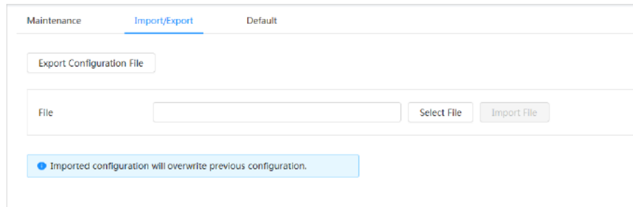
Figure 4-94 Import/export
