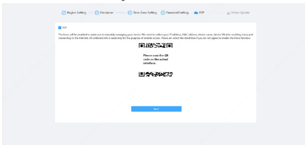
Figure 3-5 P2P
