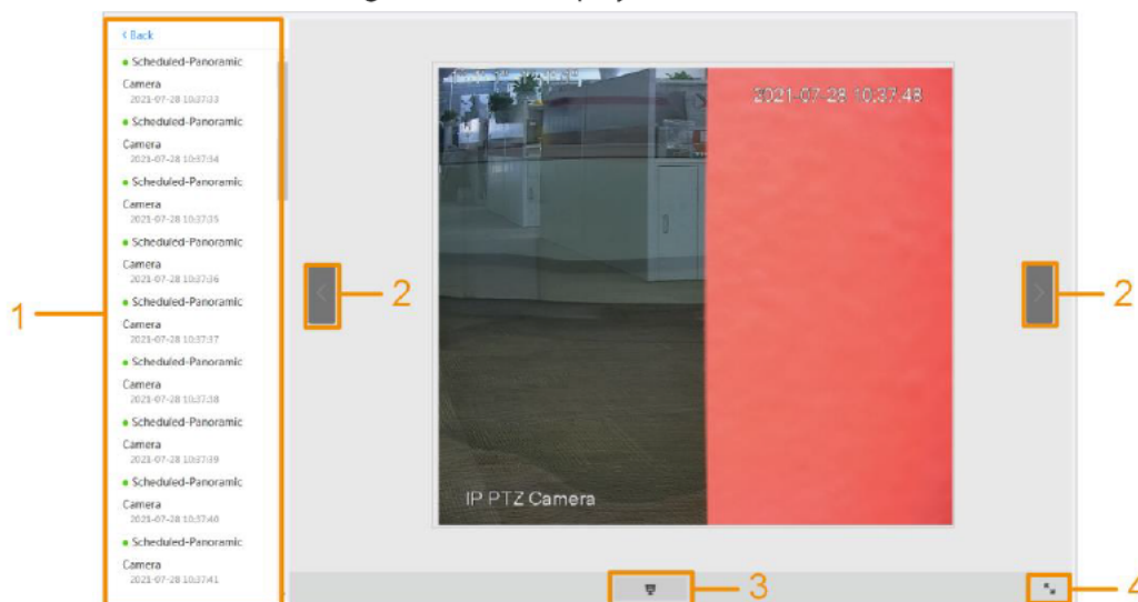
Figure 7-2 Picture playback
