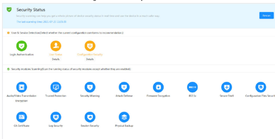
Figure 9-1 Security status
