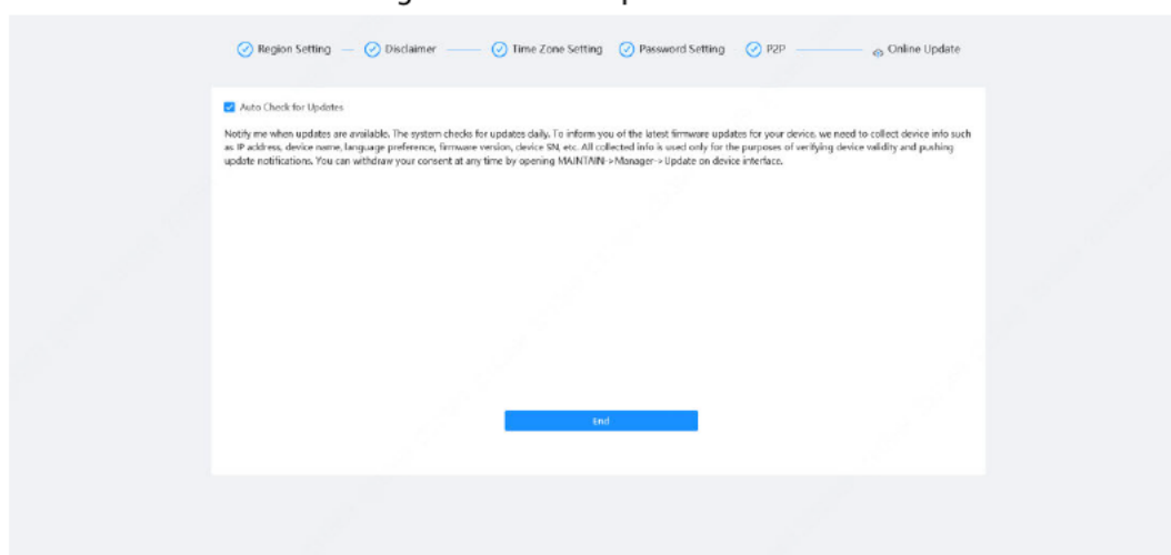
Figure 3-6 Online update
