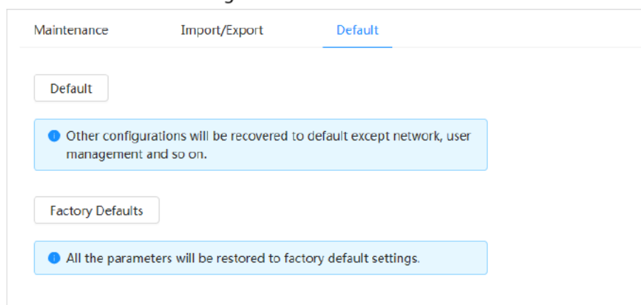
Figure 4-95 Default
