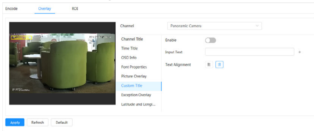
Figure 4-23 Custom title
