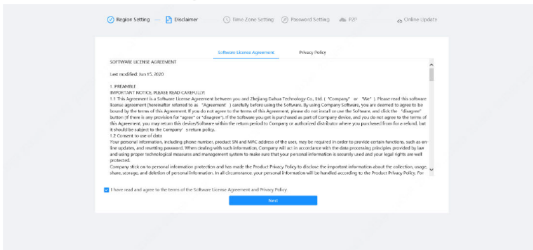
Figure 3-2 Disclaimer
