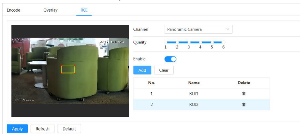
Figure 4-28 ROI
