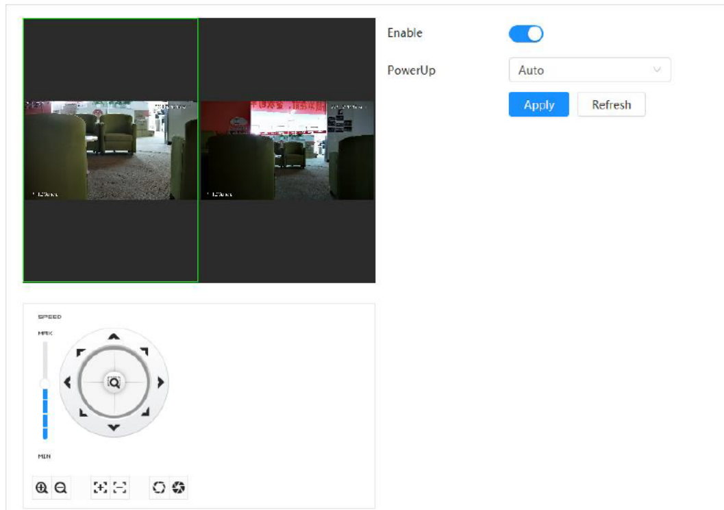
Figure 4-56 PowerUp
