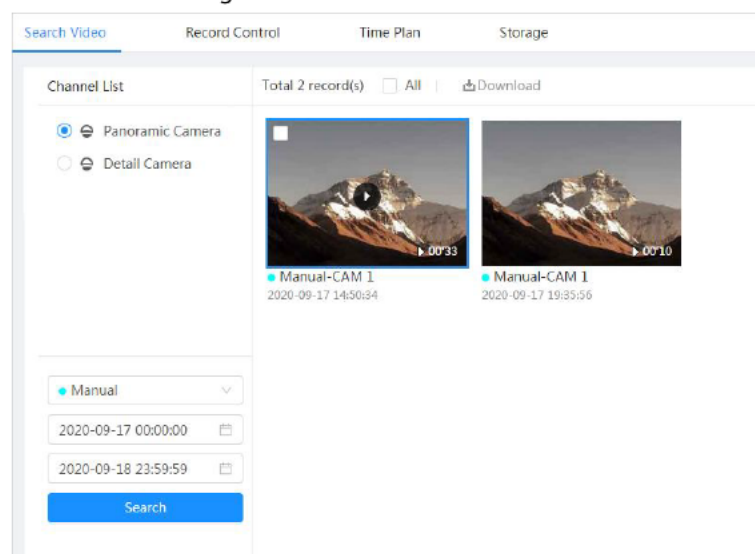
Figure 6-1 Search video
