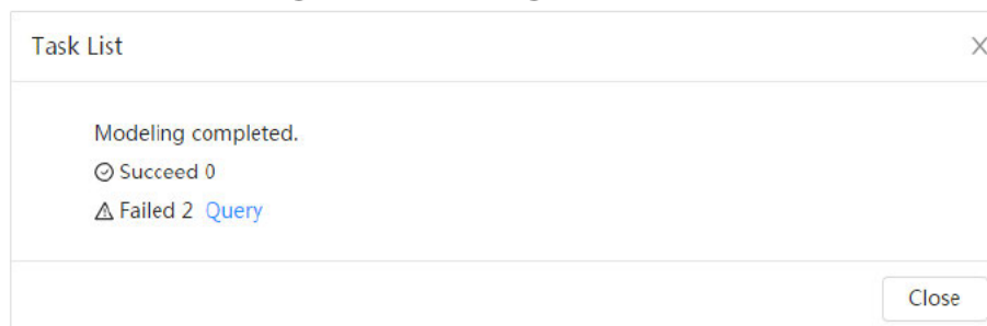
Figure 8-12 Modeling result
