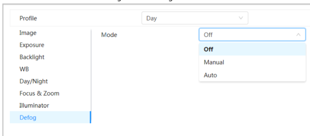
Figure 4-14 Defog
