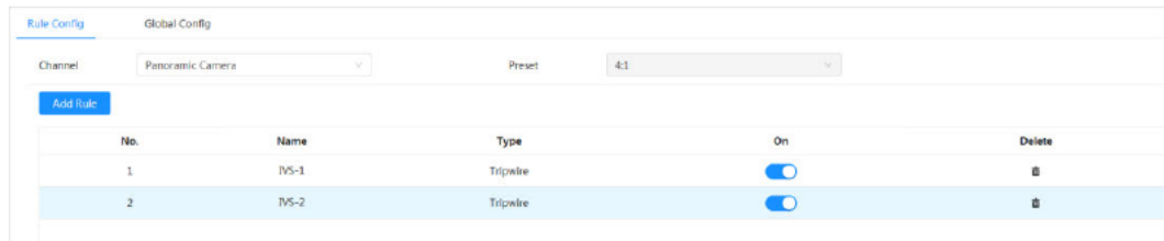
Figure 8-17 Tripwire
