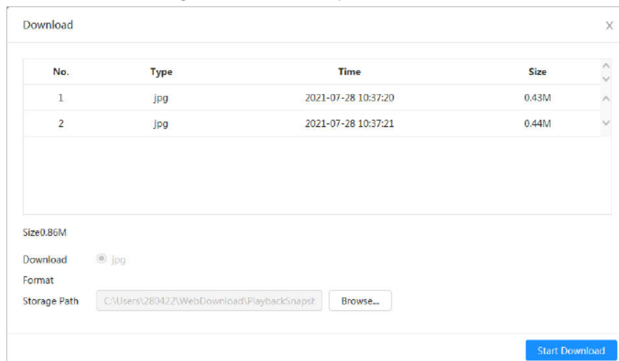
Figure 7-4 Download picture
