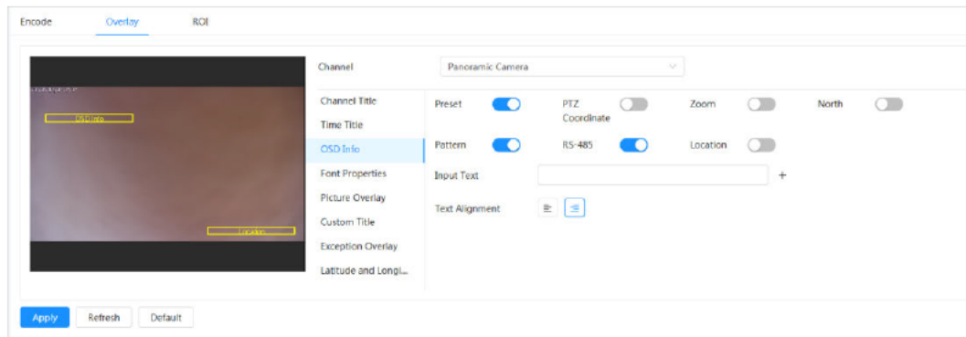
Figure 4-20 OSD info
