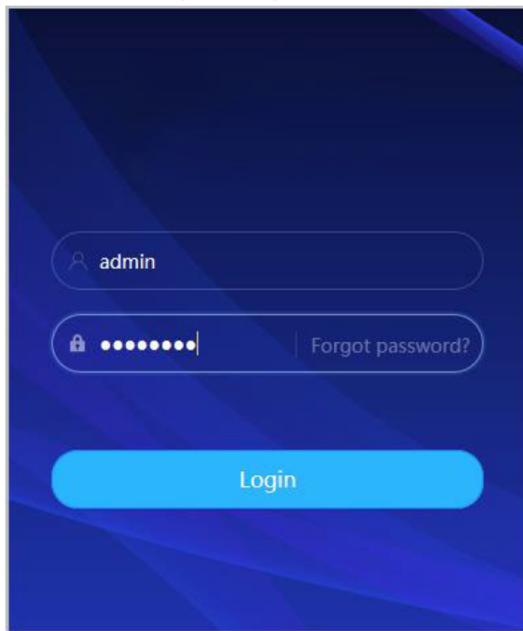
Figure 4-1 Login
