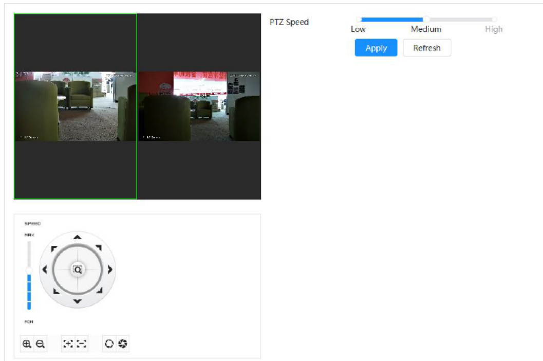
Figure 4-54 PTZ Speed
