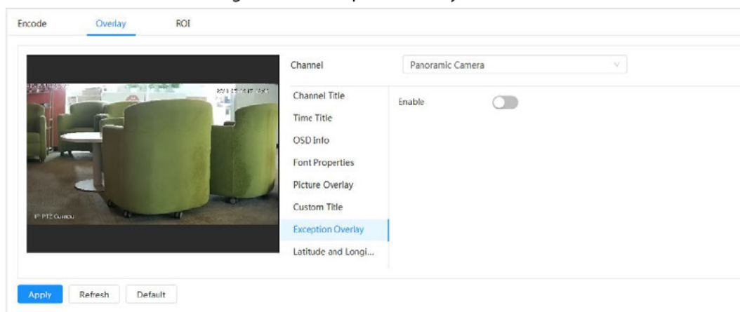
Figure 4-24 Exception overlay
