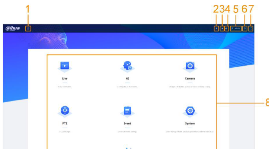
Figure 4-2 Main page
