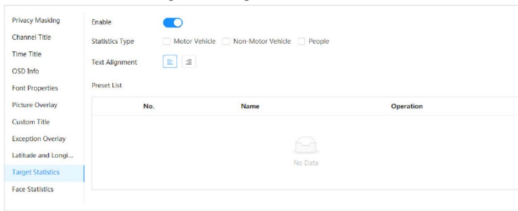
Figure 4-26 Target statistics
