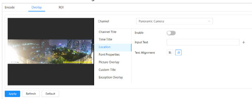
Figure 4-19 Location
