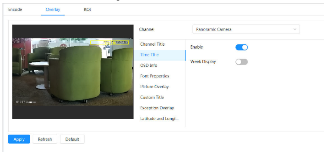
Figure 4-18 Time title
