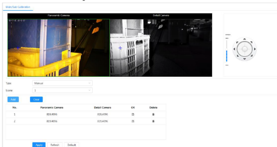
Figure 8-25 Main/sub calibration
