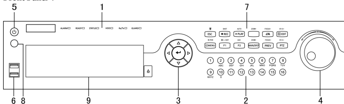
Figure 1. 4 Front Panel 4
