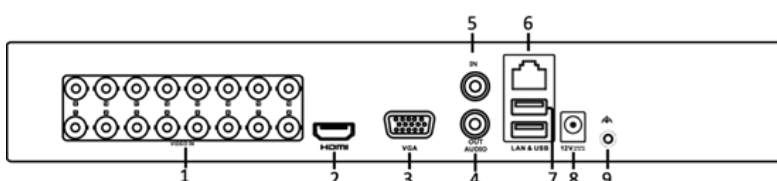
Figure 1.8 Rear Panel 1
