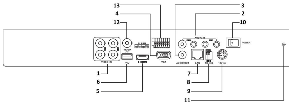
Figure 1. 4 Rear Panel
