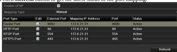
Figure 11. 16 UPnP™ Settings Finished-Manual
