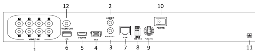
Figure 1.10 Rear Panel 3
