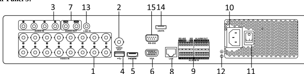
Figure 1. 12 Rear Panel 5
