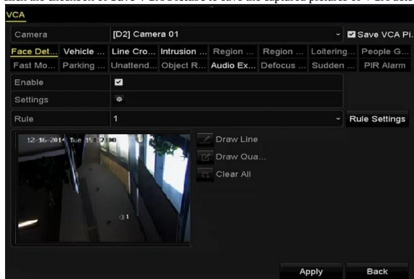
Figure 9. 1 Face Detection
