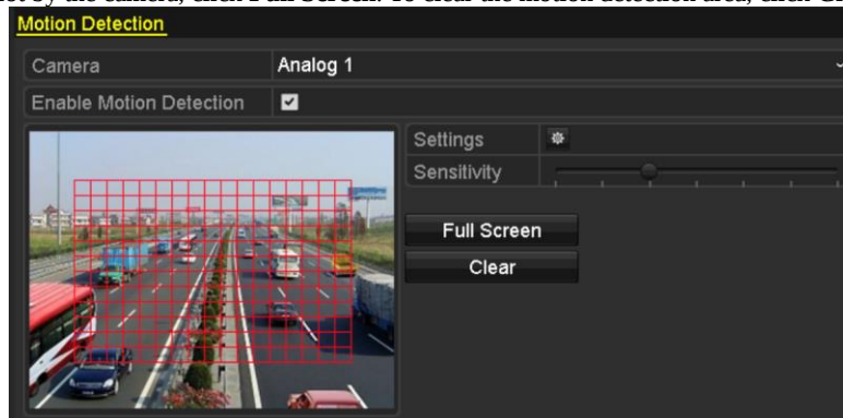
Figure 5.12 Motion Detection- Mask
