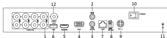
Figure 1. 5 Rear Panel 1
