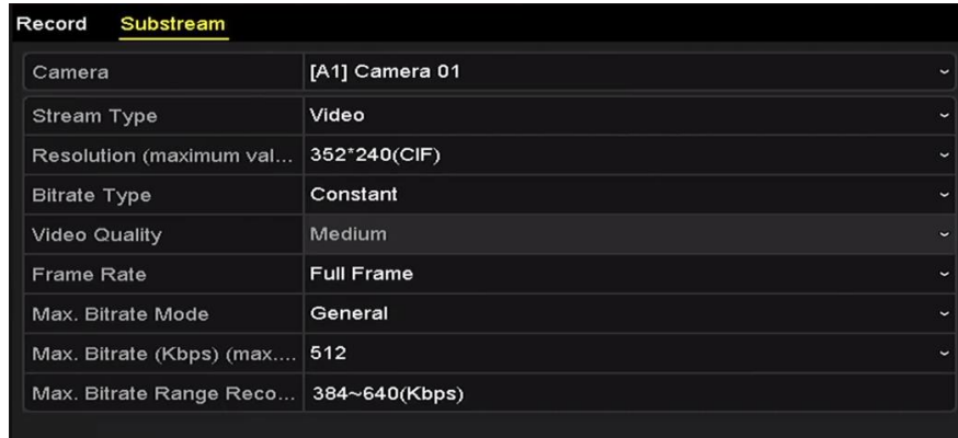
Figure 5. 6 Sub-stream Encoding
