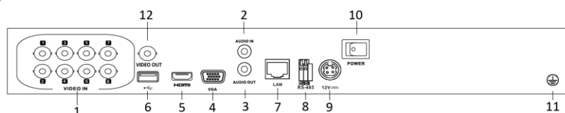
Figure 1. 6 Rear Panel 2
