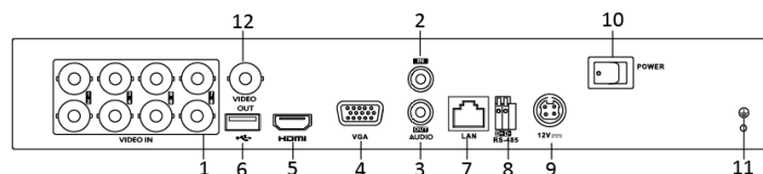
Figure 1. 5 Rear Panel 1
