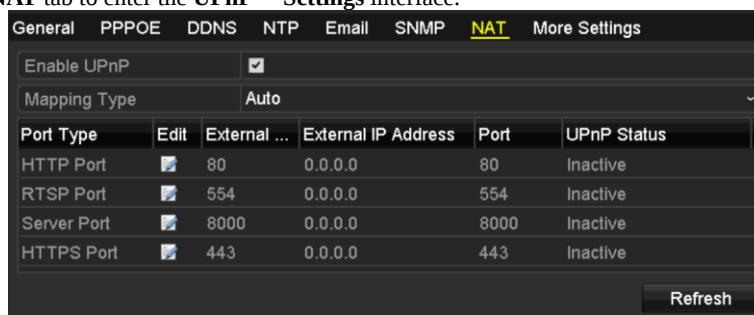
Figure 11. 12 UPnP™ Settings Interface
