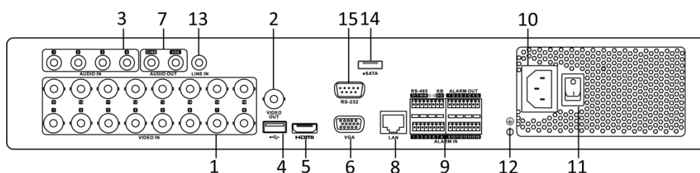
Figure 1. 8 Rear Panel 4
