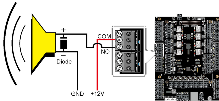
Figure 5-12 Alarm wiring
