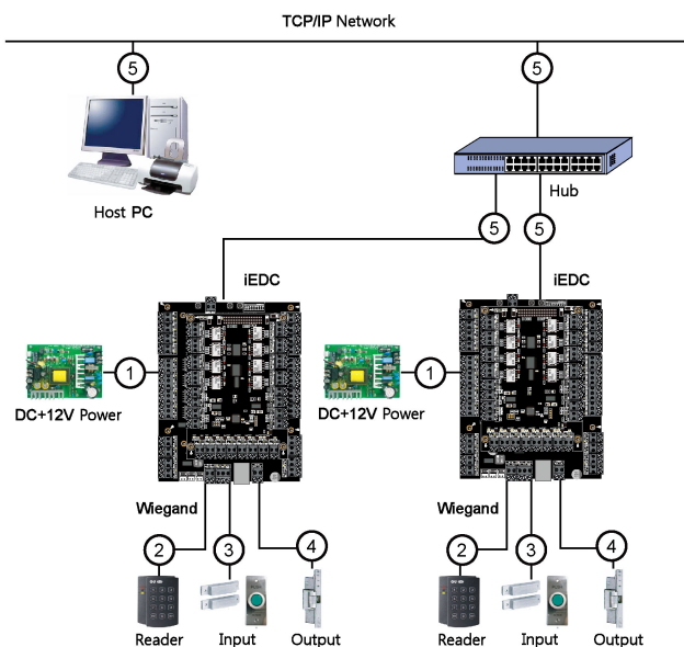
Figure 3-1 iEDC installation diagram
