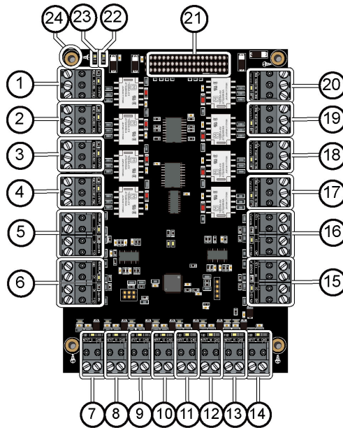
Figure 2-4 ERIO board configuration
