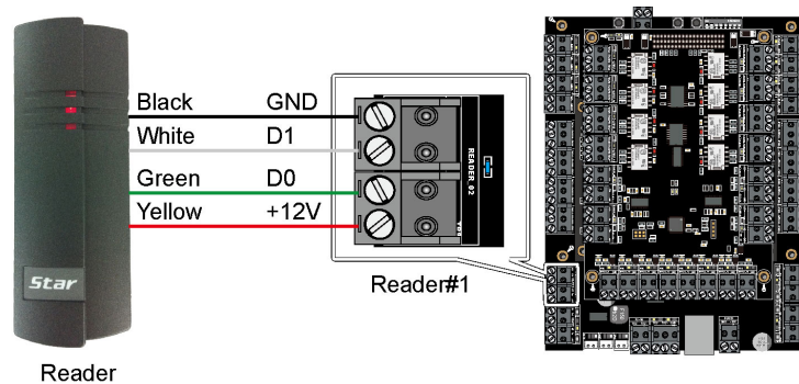
Figure 5-8 iEDC reader wiring
