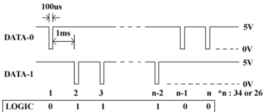
Figure 11-1 iEDC_Reader_Timing
